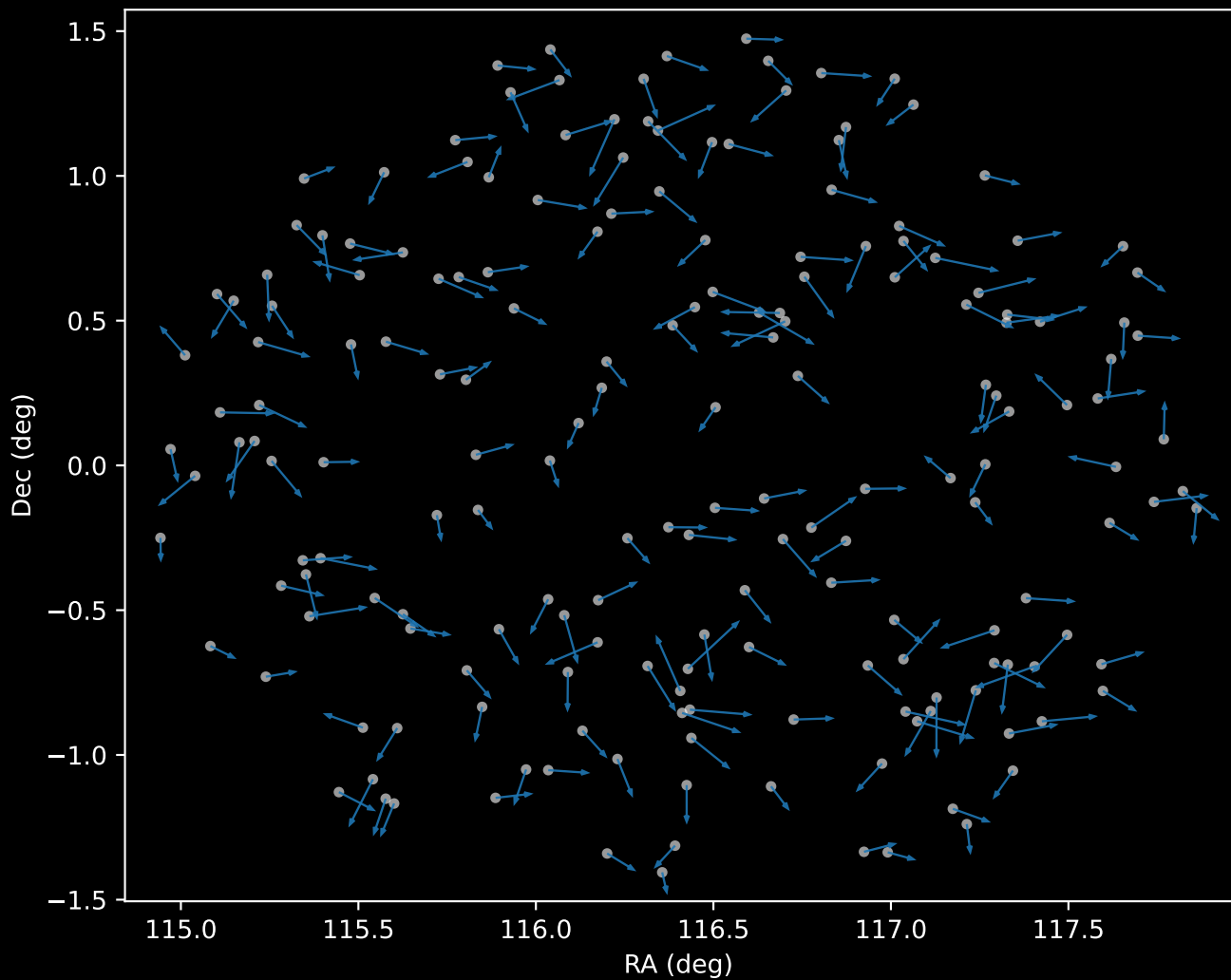
APOGEE DR17 Cluster 0 Proper Motion Vectors (n=187)
