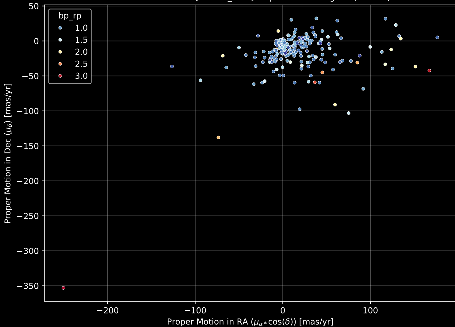
APOGEE DR17 Field: [131-63_MGA] Proper Motion Diagram (n= 209)
