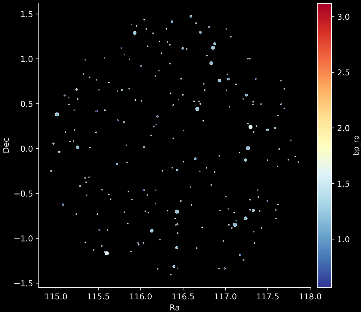
APOGEE DR17 Field: [131-63_MGA] Stars: 209
