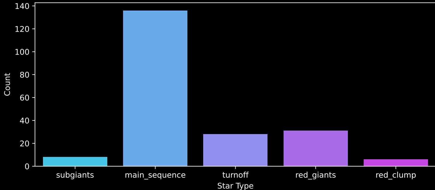
APOGEE DR17 Field: [131-63_MGA] Count plot of Star Type
