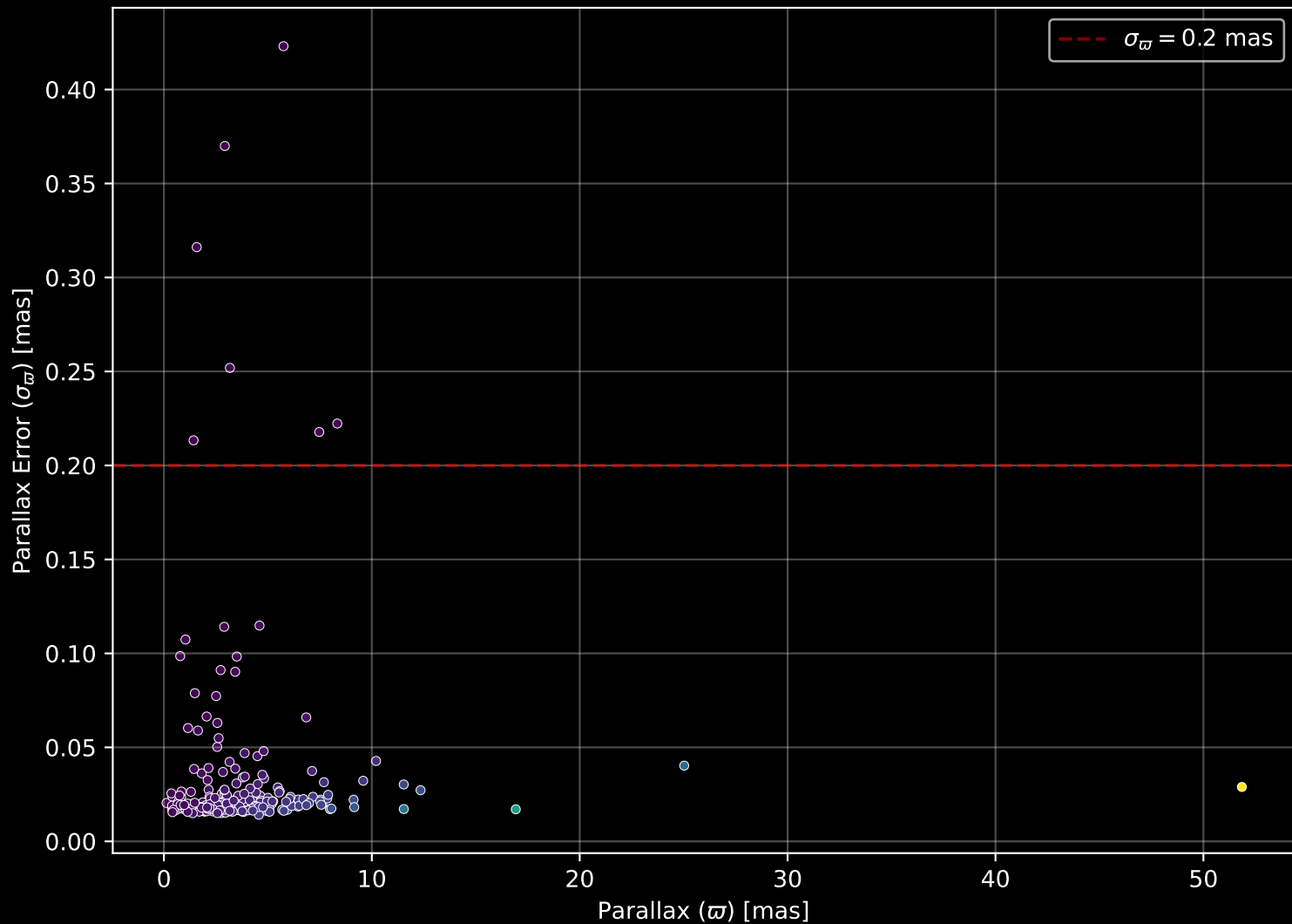
APOGEE DR17 Field: [131-63_MGA] Parallax Quality (n= 209)
