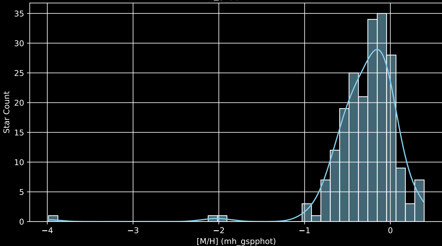
APOGEE DR17 Field: [131-63_MGA [M/H] (mh_gspphot) (n= 207)
