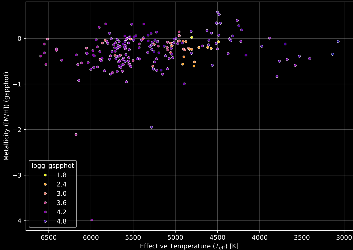
APOGEE DR17 Field: [131-63_MGA] Stellar Population Parameters (n= 209)
