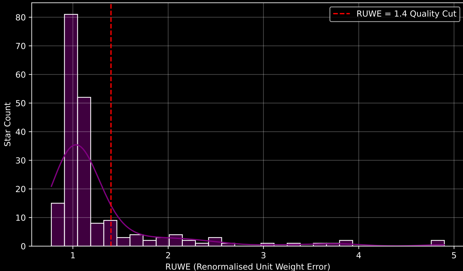
GAPOGEE DR17 Field [131-63_MGA] RUWE Distribution (n= 196)
